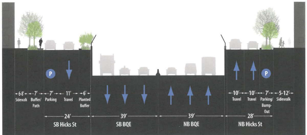
Revised geometry of Hicks Street, mid-block. From west to east: planted curbside swales and a trench-side buffer make use of the unused space on southbound Hicks; travel lanes are reallocated and a protected parking lane created on northbound Hicks.
