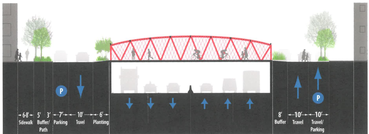
ADA-accessible ramps at chicanes and trench buffer areas create entrances for the bridges.
