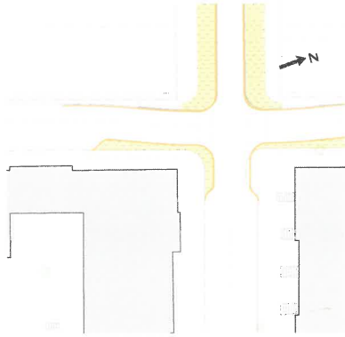
Chicane detail at Northbound Hicks Street. Extended bridge sidewalks and corner bump-outs combine to shorten pedestrian crossing distances and induce vehicles to observe speed limits.
